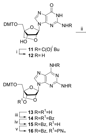
Scheme 3. Reagents and conditions: (i) Satd methanolic ammonia; (ii) (a) (TFA) 2 O, pyridine, 0 °C, (b) NH 3 (55% from 11 ); (iii) BzCl, pyridine; (iv) 2 M aq NaOH, THF, MeOH, H 2 O (6:4:1, v/v/v) (81% from 13 ); (v) NC(CH 2 ) 2 OP(N i Pr) 2 , 4,5-dicyanoimidazole, MeCN, DMF (95%). DMT = 4,4'-dimethoxytrityl, PN 2 = 2-cyanoethoxy(diisopropylamino)phosphinyl.
