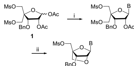
Scheme 1. (i) Vorbrüggen coupling; (ii) ring closing to form the bicyclic LNA skeleton. B = nucleobase or nucleobase analogue.
