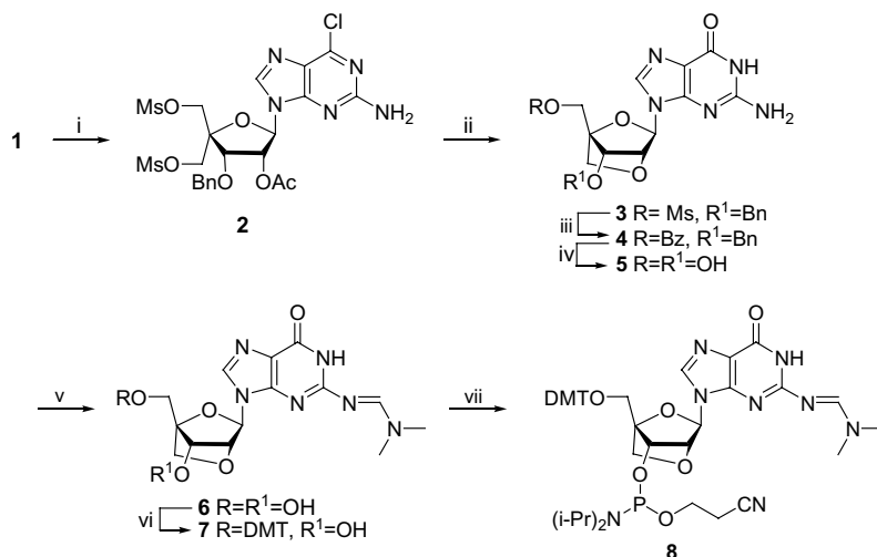
Scheme 2. Reagents and conditions: (i) 2-Amino-6-chloropurine, N,O -bis(trimethylsilyl)acetamide, TMS-triflate, 1,2-dichloroethane; (ii) HOCH 2 CH 2 CN, NaH, THF; (iii) NaOBz, DMSO, 100 °C; (iv) (a) MsOH, CH 2 Cl 2 , (b) Amberlyst A-26 (OH − (aq), EtOH); (v) (CH 3 O) 2 CHN(CH 3 ) 2 , (vi) DMT-Cl, pyridine (vii) NC(CH 2 ) 2 OP(N (i Pr) 2 ) 2 , 4,5-dicyanoimidazole, MeCN, CH 2 Cl 2 . DMT = 4,4'-dimethoxytrityl.
