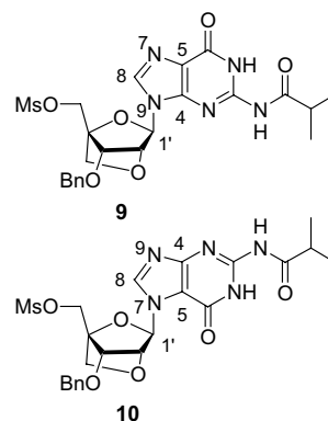
Figure 2. The N9 isomer ( 9 ) and the N7 isomer ( 10 ).
