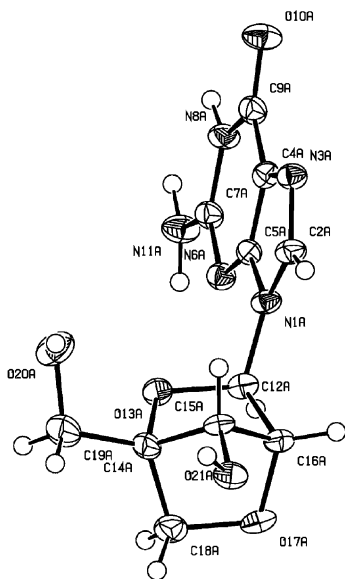
Figure 1. X-ray structure of nucleoside 5.
