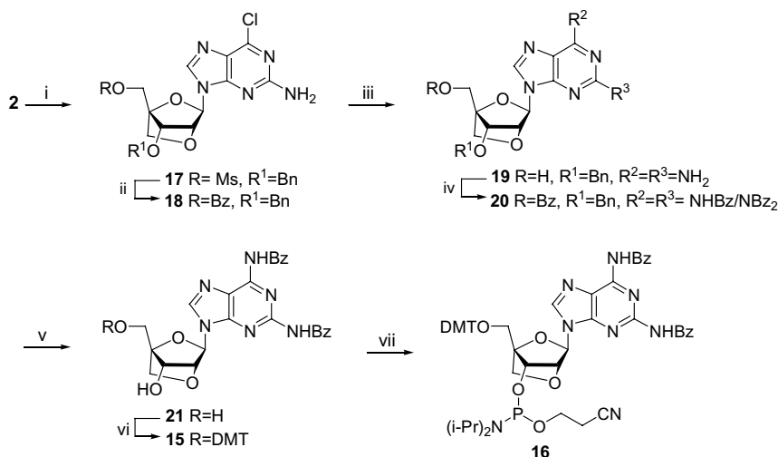
Scheme 4. Reagents and conditions: (i) LiOH (aq), THF; (ii) BzONa, DMF; (iii) satd methanolic ammonia (80 °C/60 psi); (iv) BzCl, pyridine; (v) (a) MsOH, CH 2 Cl 2 , (b) Amberlyst A-26 (OH - , aq); (vi) DMT-Cl, pyridine (vii) NC(CH 2 ) 2 OP(N i Pr) 2 , 4,5-dicyanoimidazole, MeCN, DMF. DMT = 4,4'-dimethoxytrityl.
